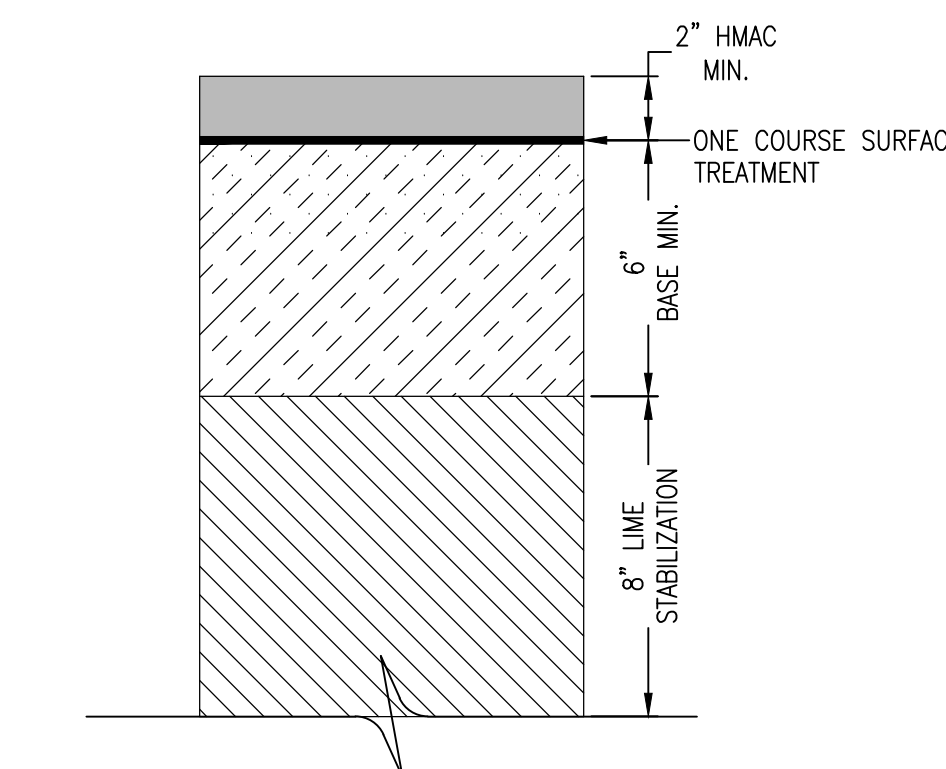
PRELIMINARY PAVEMENT SECTION
