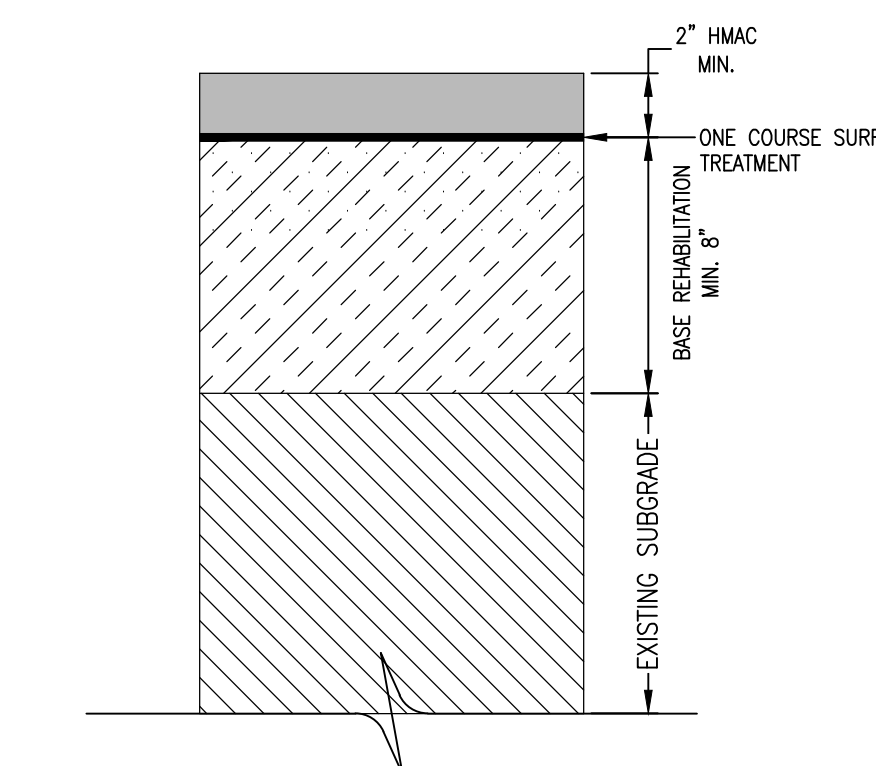
PRELIMINARY PAVEMENT SECTION
