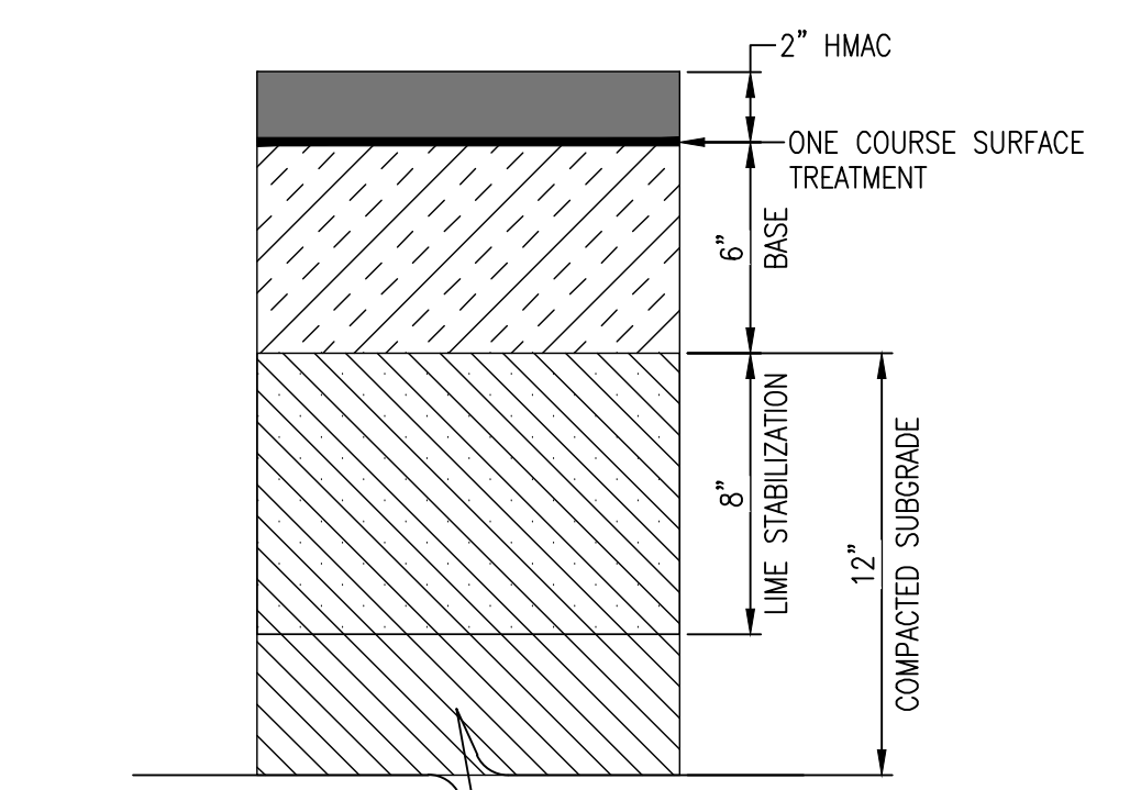
PRELIMINARY PAVEMENT SECTION
