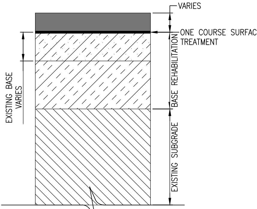
PRELIMINARY PAVEMENT SECTION
