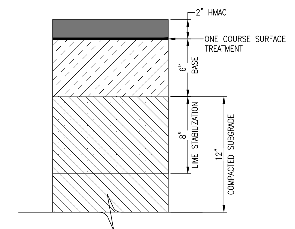
PRELIMINARY PAVEMENT SECTION
