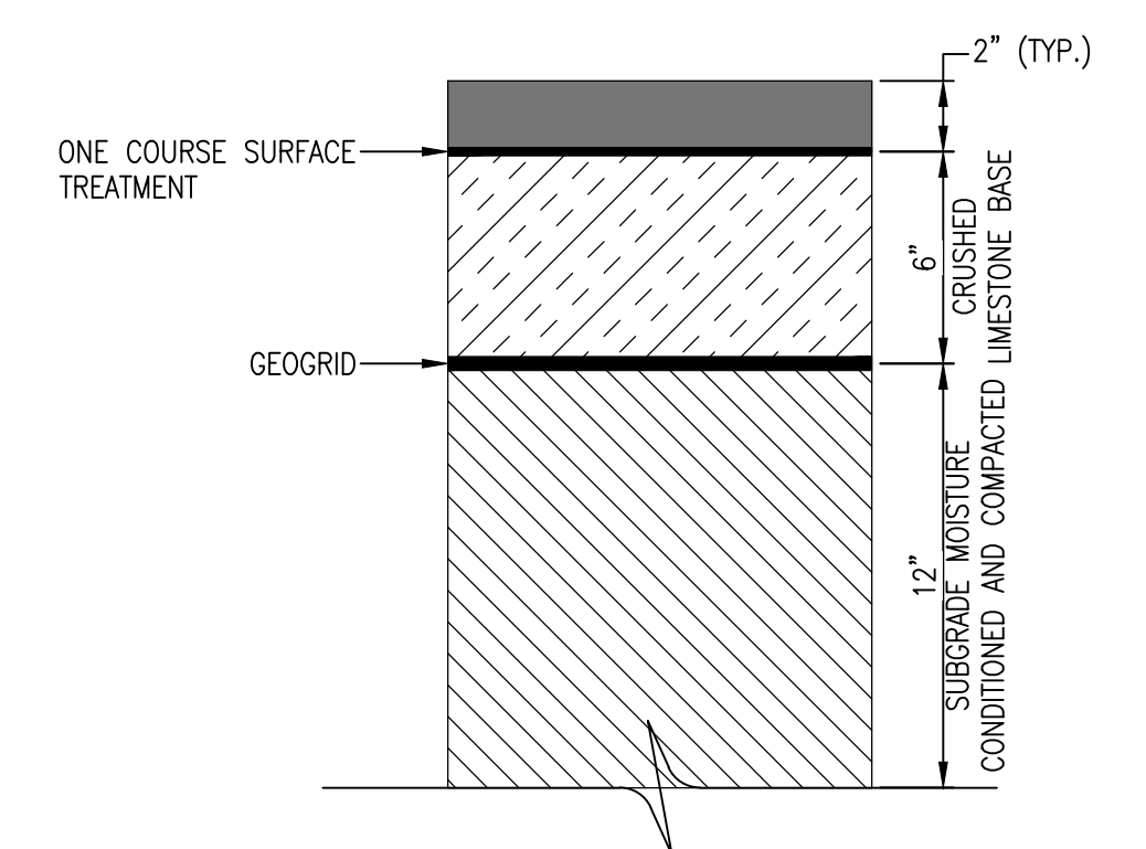
PRELIMINARY PAVEMENT SECTION
